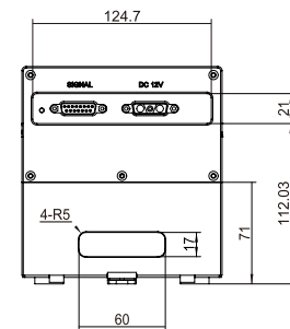
AONano Compact-532 (water cooling) Laser CAD Drawing
